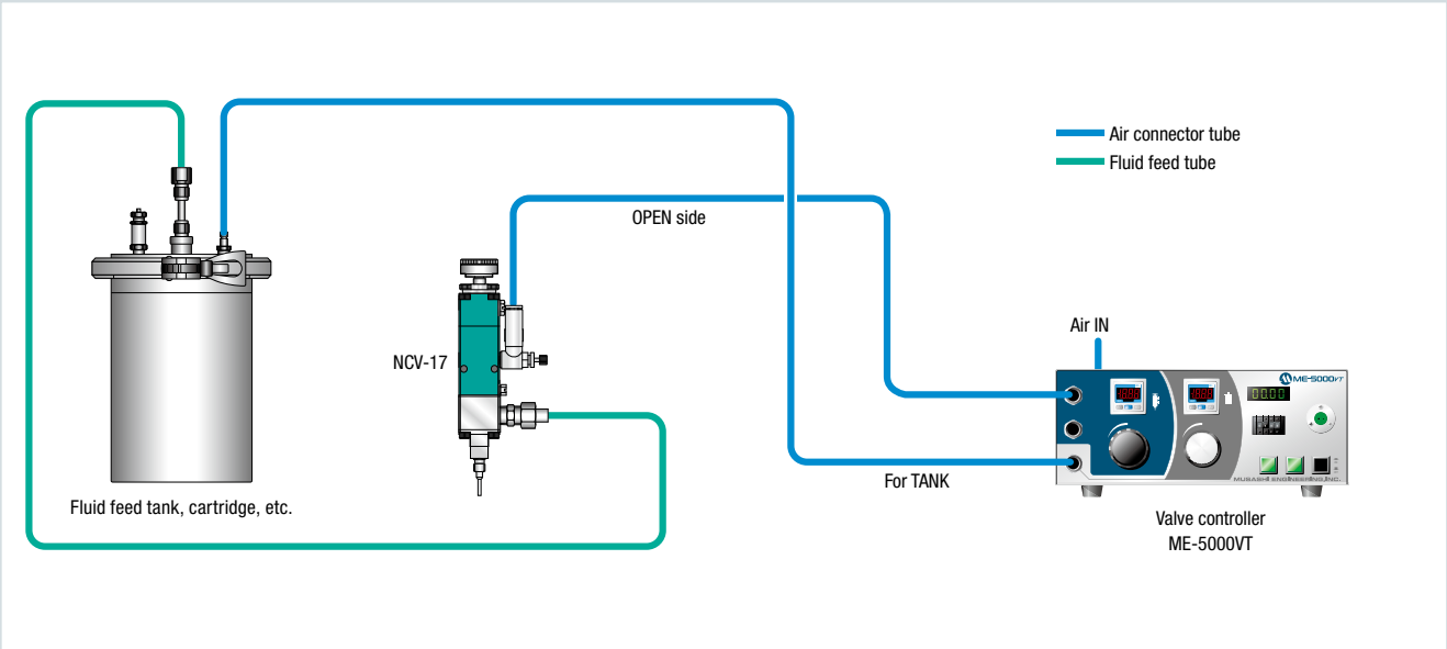
Configuration diagram of the valve and tank system
