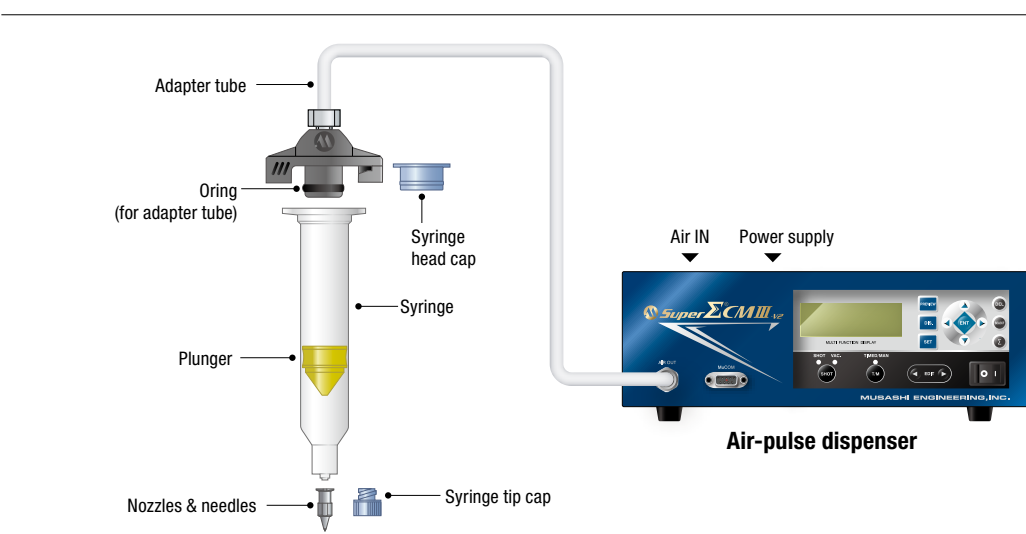
Air-pulse dispenser Syringe Connection System Configuration Chart
